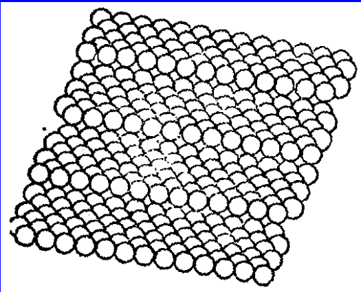
fcc(775)
