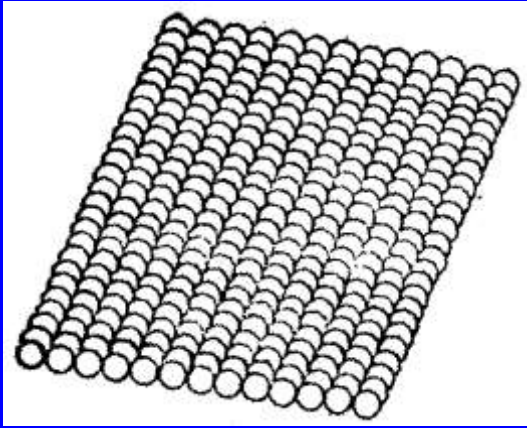
fcc(100)
