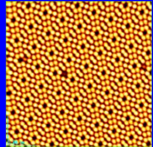
STM image of Si(111) 7x7 surface
