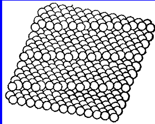
fcc(10 8 7)
