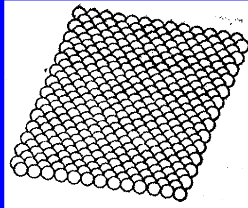
fcc(111)
